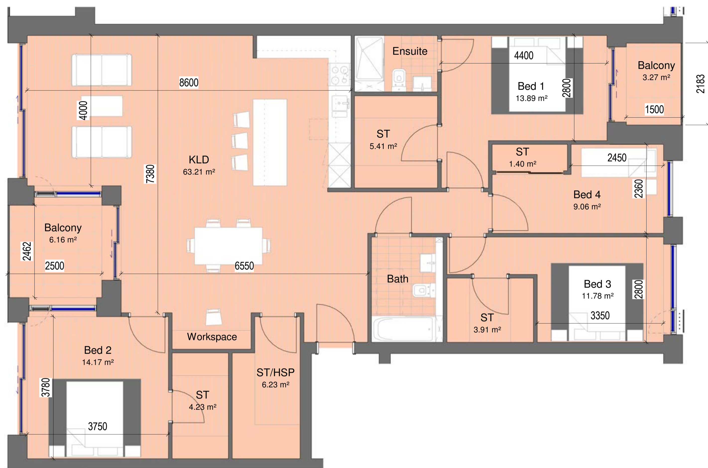
Block D_4 Bedroom Apartment Type 01 1 : 50 Size: 147.3m 2 Total Apartments: 1
