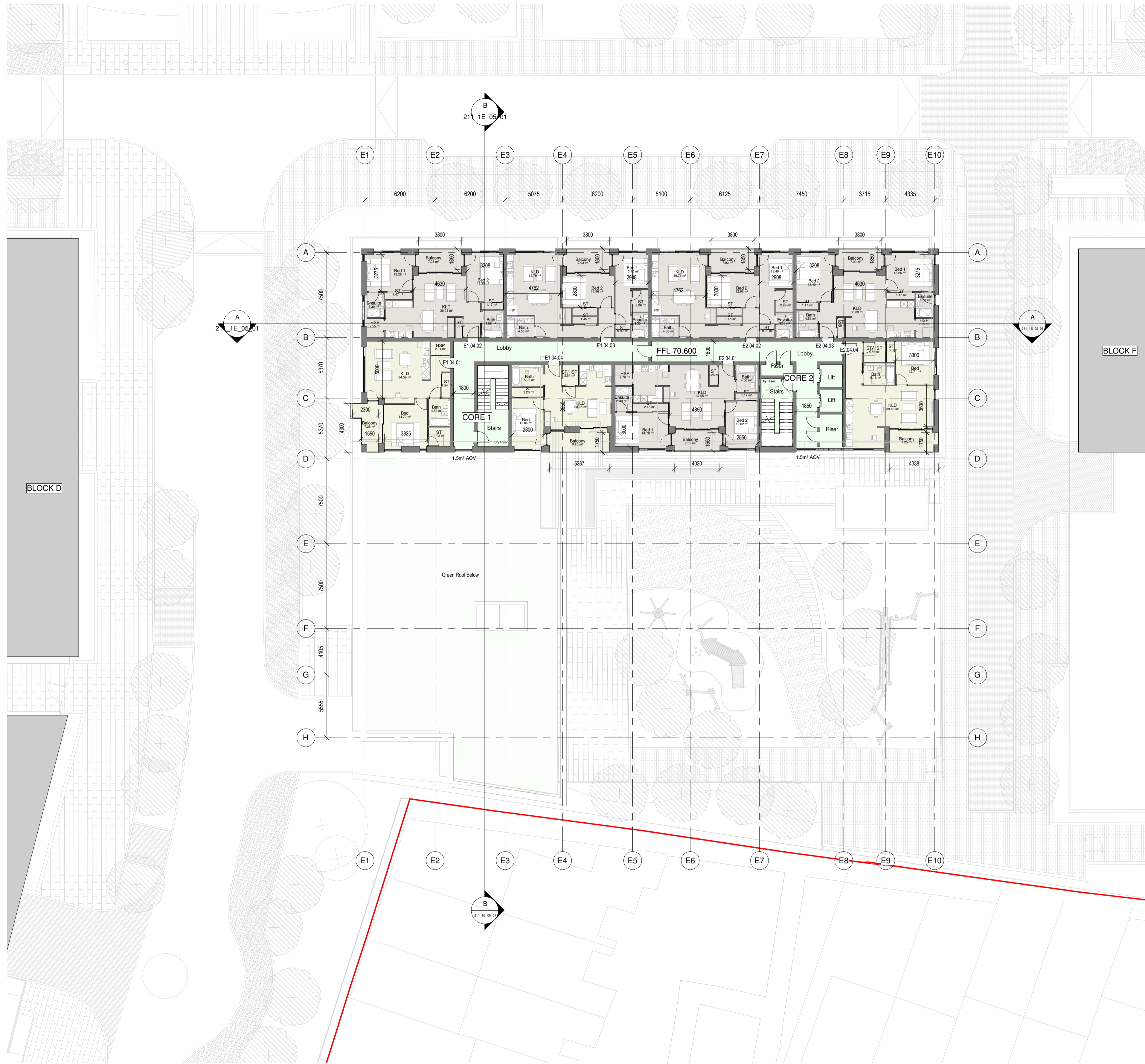
Block 1E_Fourth Floor Plan 1 : 200
