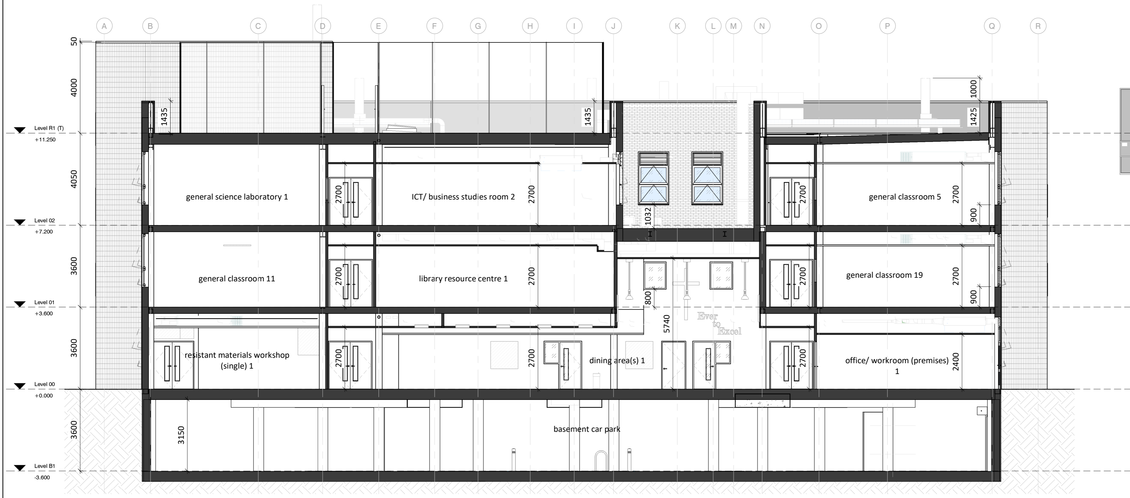
0402 - Main School - Building Section C 1:100
