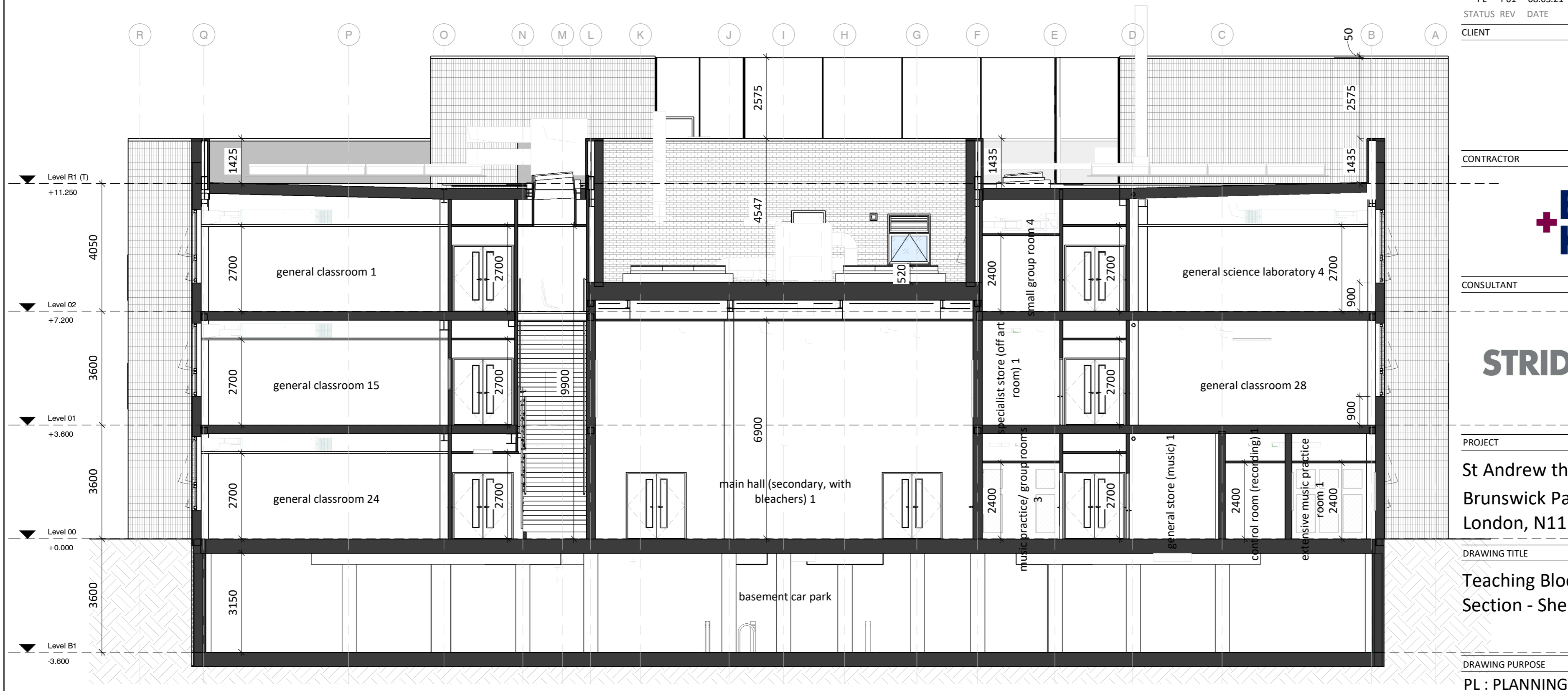
0402 - Main School - Building Section E 1:100
