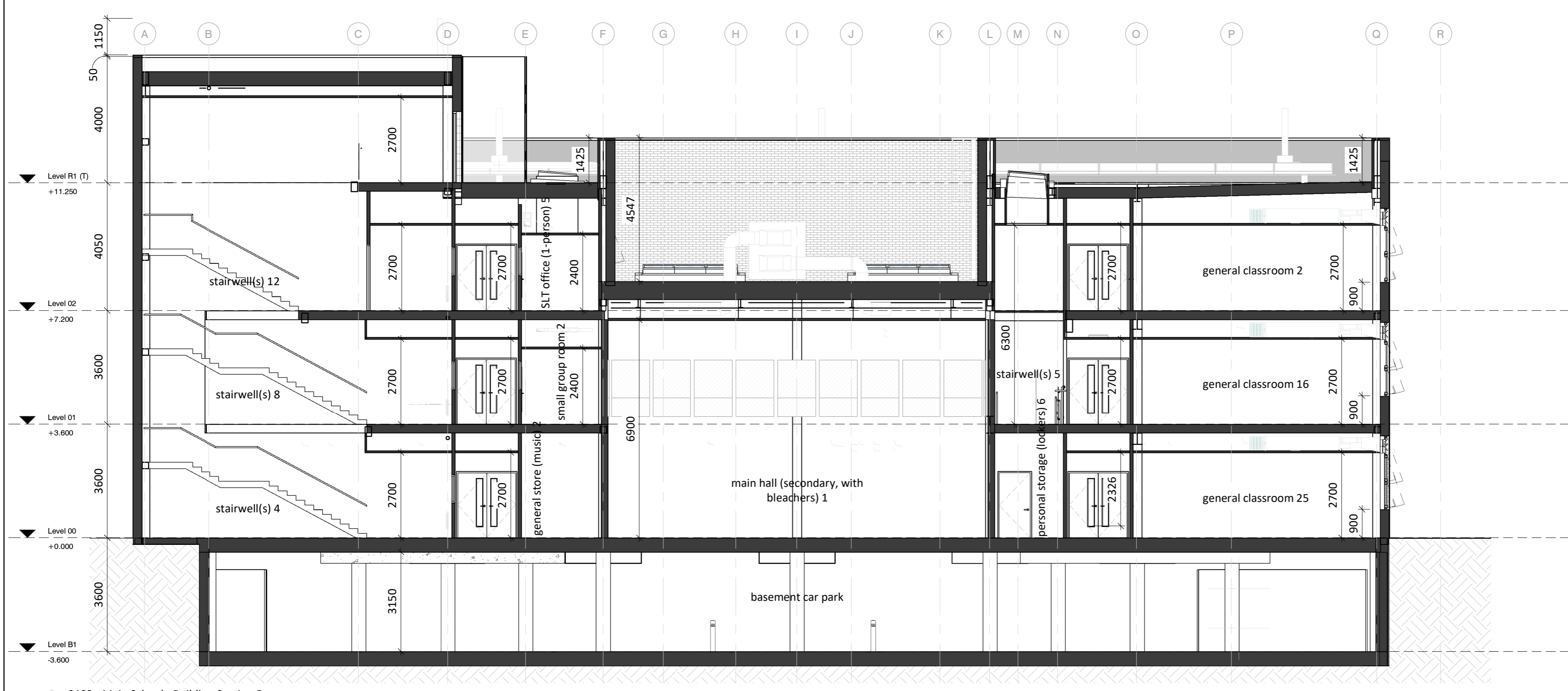
0402 - Main School - Building Section D 1:100
