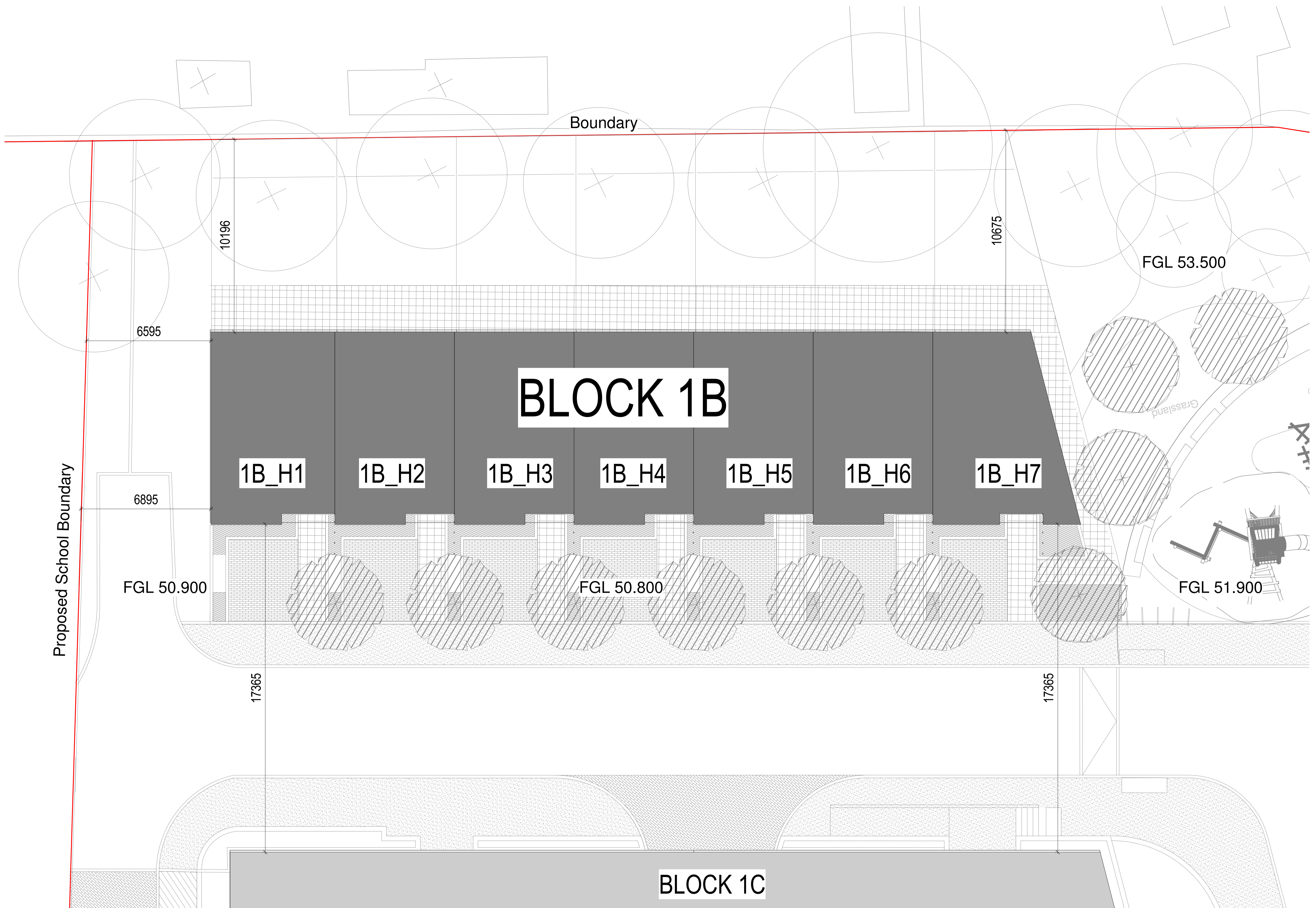
1 Block 1B_Site Plan 1 : 100
