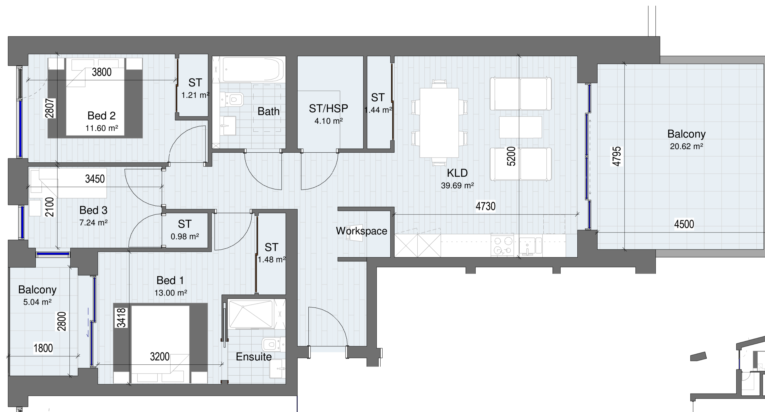
1 Block C_3 Bedroom Apartment type 01 1 : 50 Size: 94.1m 2 Total Apartments: 1
