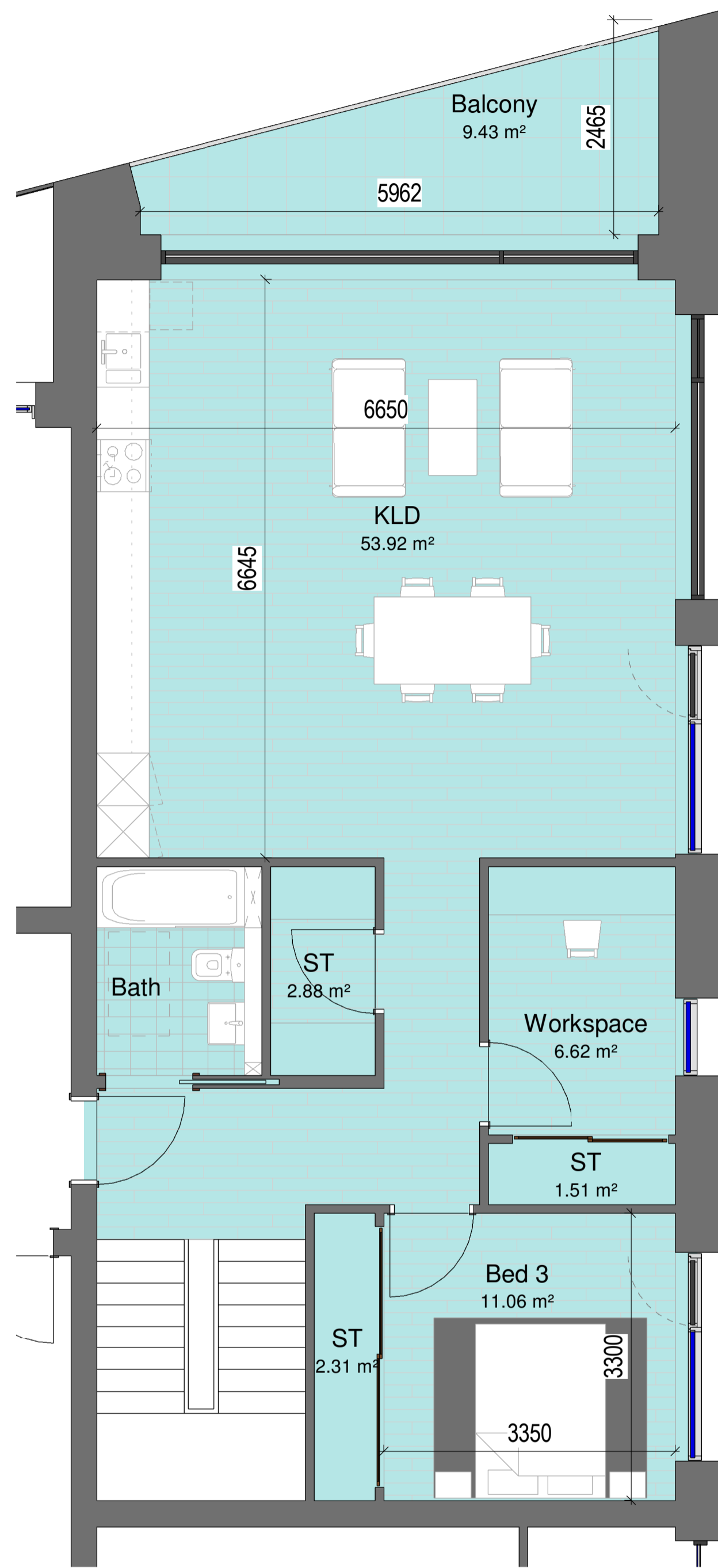
1 Block C_3 Bedroom Duplex Apartment Type 01 1 : 50
