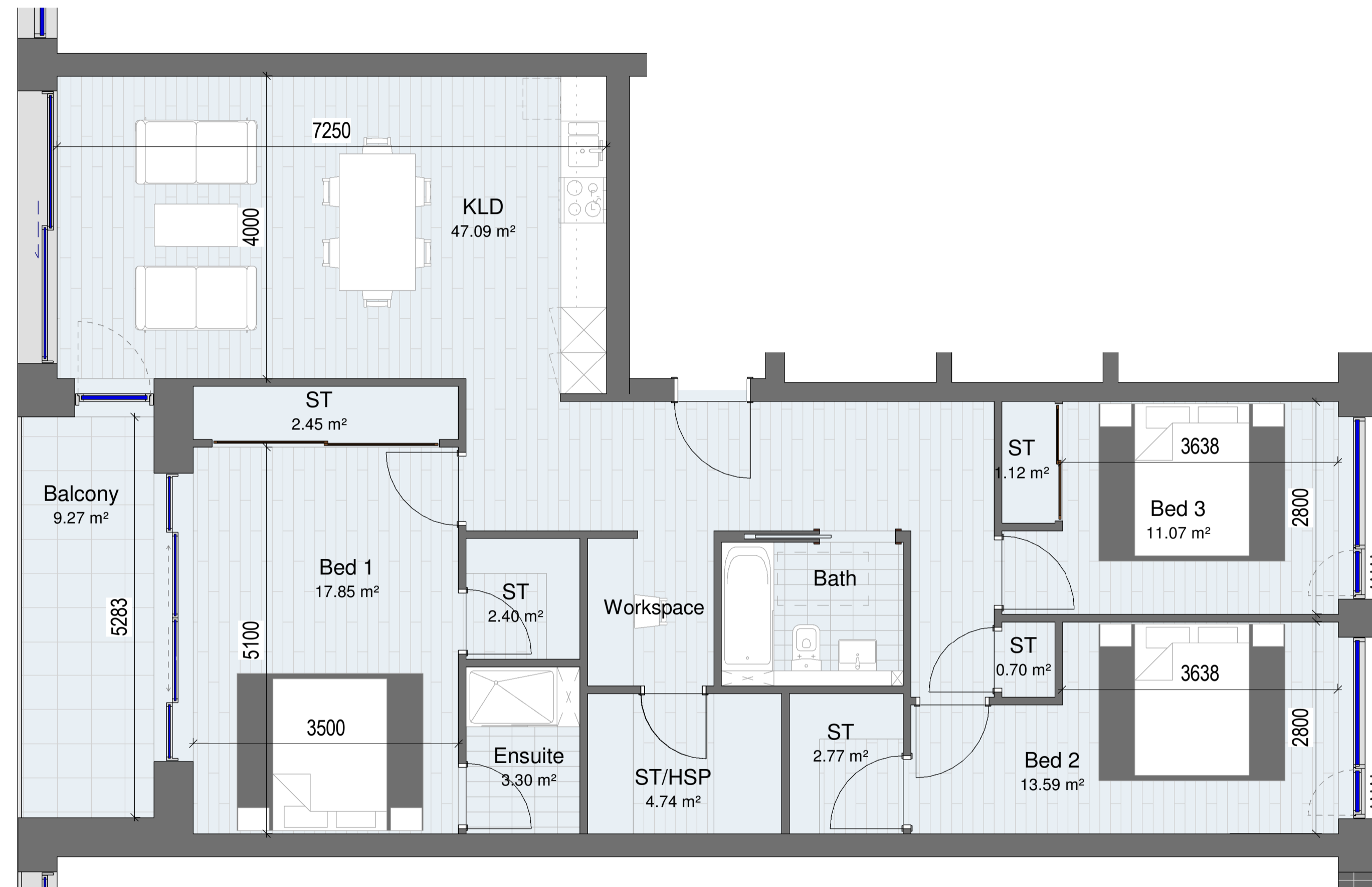
1 Block D_3 Bedroom Apartment Type 05 1 : 50 Size: 116.7m 2 Total Apartments: 8
