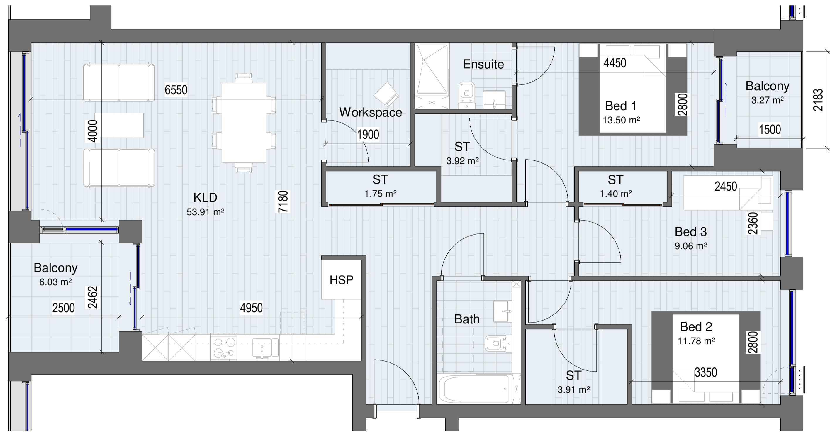
1 Block D_3 Bedroom Apartment Type 06 1 : 50 Size: 118.2m 2 Total Apartments: 8
