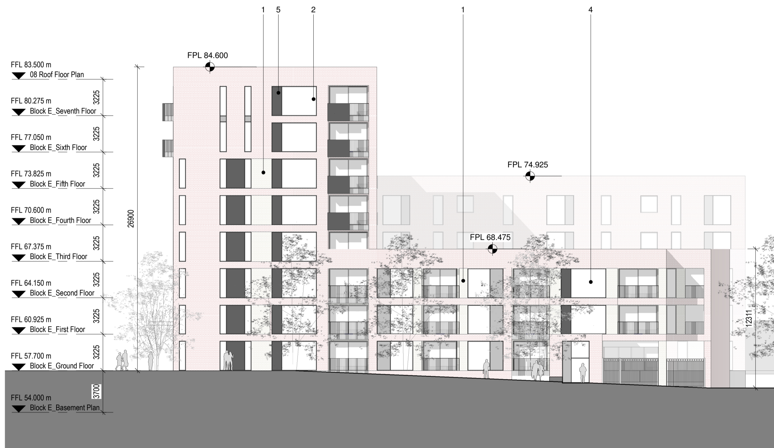
1 Block 1E_South Elevation 1 : 200
