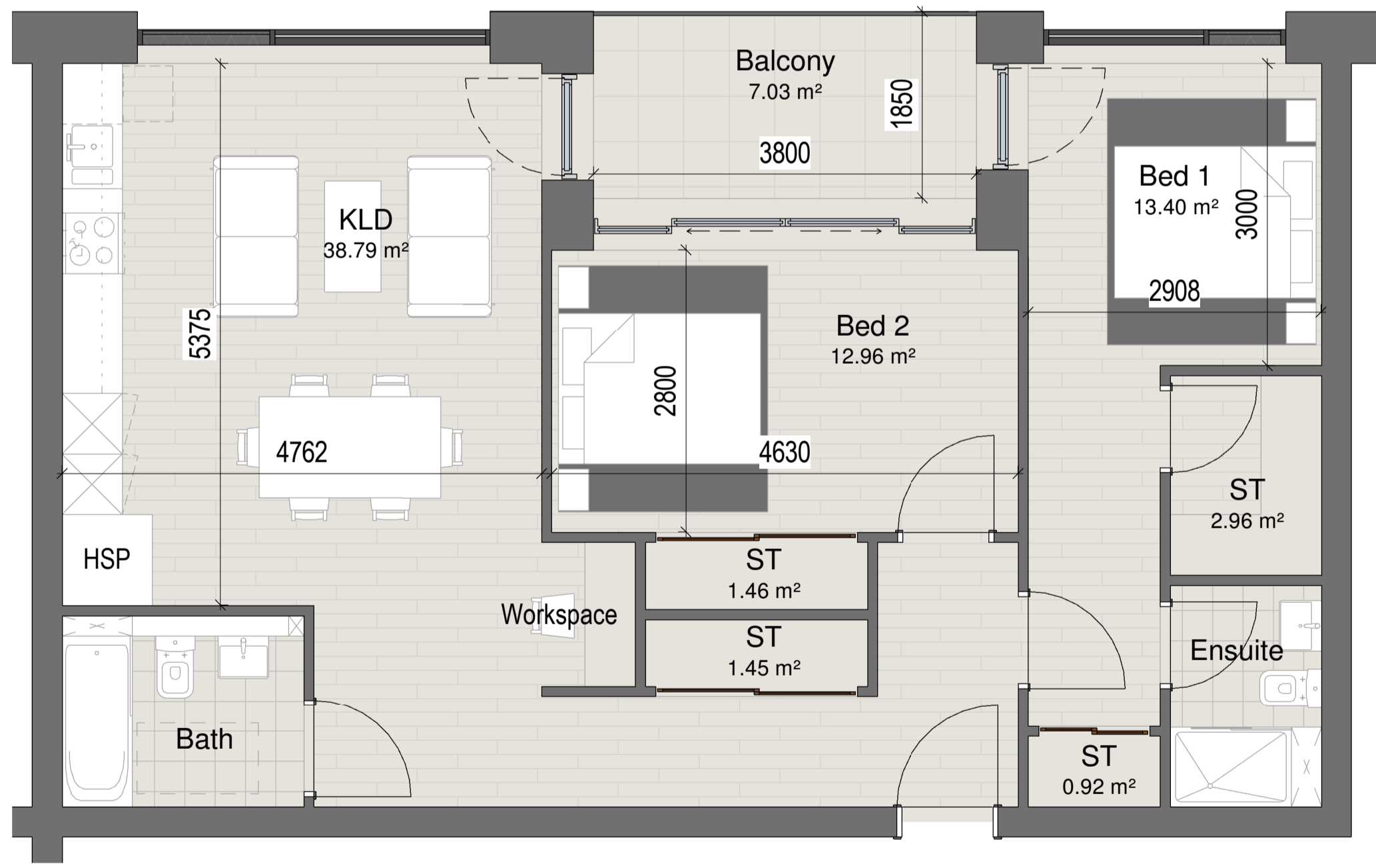
2 Block E_2 Bedroom Apartment type 02 1 : 50 Size: 83.3m 2 Total Apartments: 12
