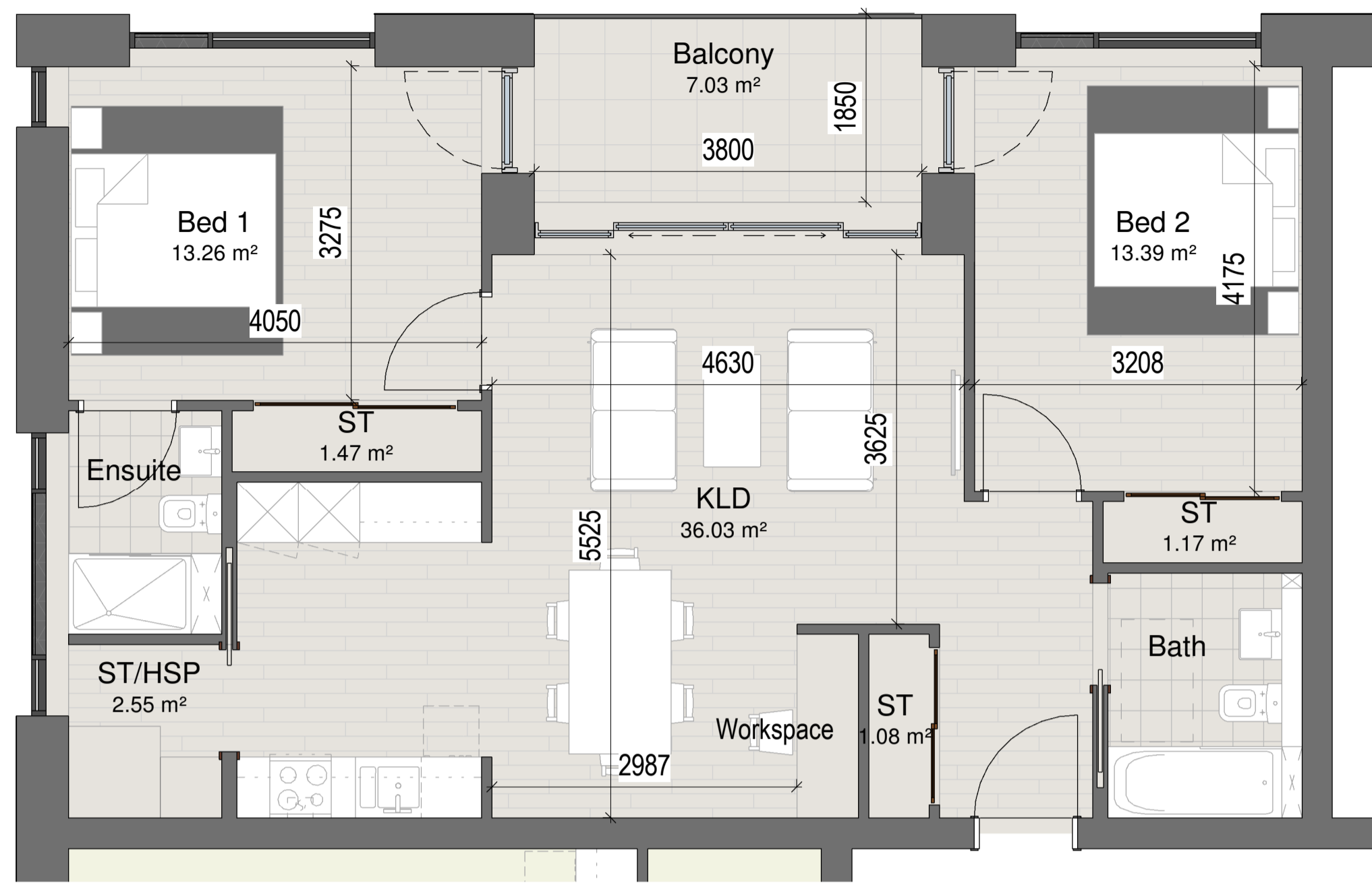
1 Block E_2 Bedroom Apartment type 01 1 : 50 Size: 80.2m 2 Total Apartments: 13
