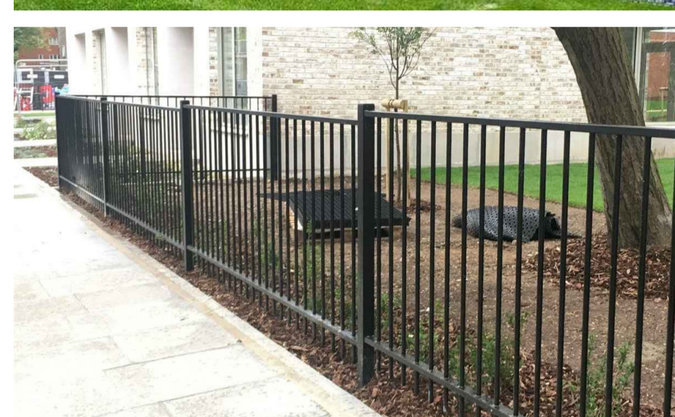
3 Townhouse Railings Nts Product: Sentry Residential Railings Manufacturer: Jacksons Fencing Height: 1.25m high Gate: not required
